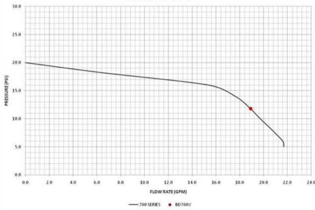
700 SERIES PERFORMANCE CURVE
